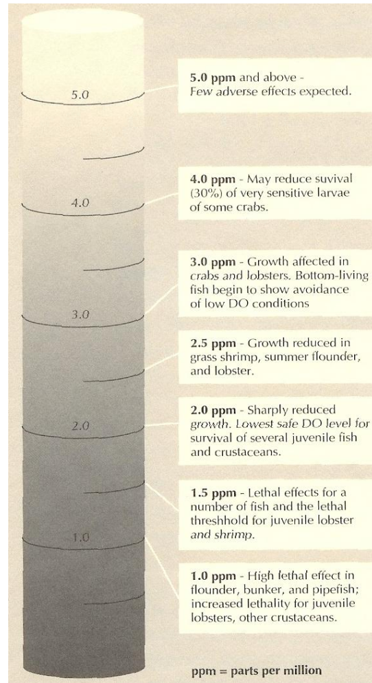
Figure 1. Effect of depleted DO on marine life (Source: Hempstead Harbor, Its History, Ecology, and Environmental Challenges, 1998)
