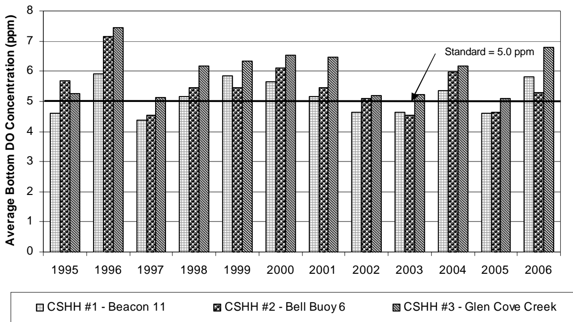
Figure 2. Measured average DO in Hempstead Harbor for 12 monitoring seasons
